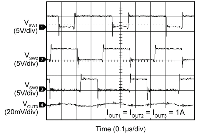
Switching Waveform (All Channels in Continuous Mode)
